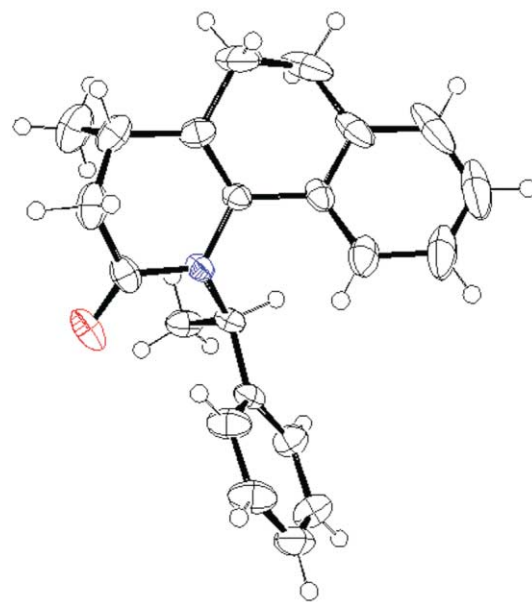
Figure 3. X-Ray structure of the major adduct 7a .
