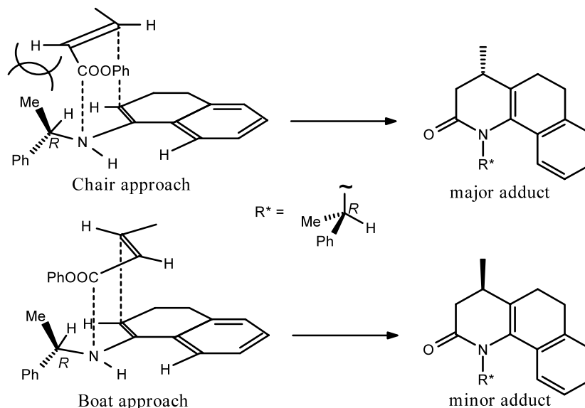
Figure 4. Possible transition states of the Michael reaction.
